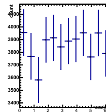
Raw Yields 1/5 < y < 2/5 , 3.5/4.5 < \cos(\theta^*) < 4.5/4.5
