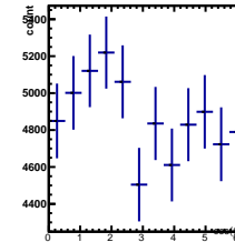
Raw Yields -2/5 < y < -1/5, -1.5/4.5 < \cos(\theta^*) < -0.5/4.5
