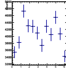
Raw Yields -3/5 < y < -2/5 , 2.5/4.5 < \cos(\theta^*) < 3.5/4.5
