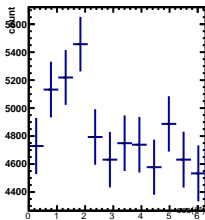
Raw Yields -2/5 < y < -1/5, -0.5/4.5 < \cos(\theta^*) < 0.5/4.5
