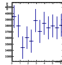
Raw Yields 1/5 < y < 2/5, -4.5/4.5 < \cos(\theta^*) < -3.5/4.5
