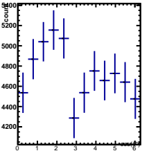
Raw Yields -2/5 < y < -1/5, 0.5/4.5 < \cos(\theta^*) < 1.5/4.5
