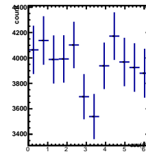
Raw Yields -3/5 < y < -2/5, -4.5/4.5 < \cos(\theta^*) < -3.5/4.5
