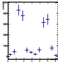
Raw Yields -5/5 < y < -4/5, -0.5/4.5 < \cos(\theta^*) < 0.5/4.5
