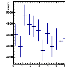
Raw Yields -1/5 < y < 0/5, -1.5/4.5 < \cos(\theta^*) < -0.5/4.5
