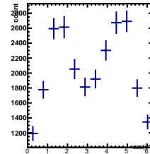
Raw Yields -4/5 < y < -3/5 , 2.5/4.5 < \cos(\theta^*) < 3.5/4.5
