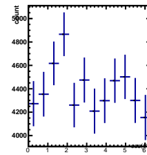
Raw Yields -1/5 < y < 0/5, -2.5/4.5 < \cos(\theta^*) < -1.5/4.5
