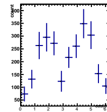
Raw Yields 4/5 < y < 5/5, -4.5/4.5 < \cos(\theta^*) < -3.5/4.5
