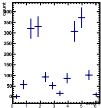
Raw Yields -5/5 < y < -4/5, 0.5/4.5 < \cos(\theta^*) < 1.5/4.5
