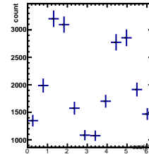
Raw Yields -4/5 < y < -3/5, -1.5/4.5 < \cos(\theta^*) < -0.5/4.5
