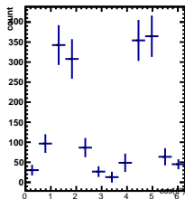
Raw Yields 4/5 < y < 5/5, -0.5/4.5 < \cos(\theta^*) < 0.5/4.5
