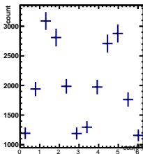
Raw Yields 3/5 < y < 4/5, -0.5/4.5 < \cos(\theta^*) < 0.5/4.5
