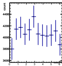
Raw Yields 0/5 < y < 1/5, -3.5/4.5 < \cos(\theta^*) < -2.5/4.5
