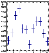
Raw Yields 2/5 < y < 3/5, -0.5/4.5 < \cos(\theta^*) < 0.5/4.5
