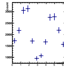
Raw Yields -4/5 < y < -3/5, -2.5/4.5 < \cos(\theta^*) < -1.5/4.5
