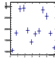
Raw Yields 3/5 < y < 4/5, -2.5/4.5 < \cos(\theta^*) < -1.5/4.5
