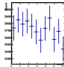
Raw Yields 0/5 < y < 1/5 , 3.5/4.5 < \cos(\theta^*) < 4.5/4.5
