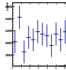
Raw Yields -2/5 < y < -1/5, -4.5/4.5 < \cos(\theta^*) < -3.5/4.5
