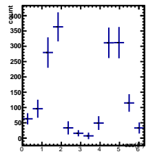
Raw Yields -5/5 < y < -4/5, -2.5/4.5 < \cos(\theta^*) < -1.5/4.5
