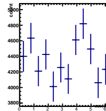
Raw Yields -2/5 < y < -1/5, -3.5/4.5 < \cos(\theta^*) < -2.5/4.5
