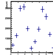
Raw Yields 3/5 < y < 4/5, -1.5/4.5 < \cos(\theta^*) < -0.5/4.5
