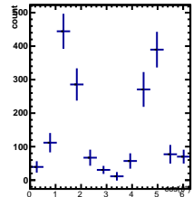
Raw Yields 4/5 < y < 5/5 , 1.5/4.5 < \cos(\theta^*) < 2.5/4.5
