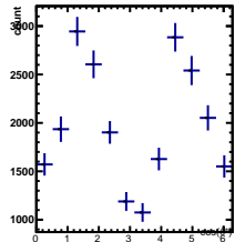
Raw Yields 3/5 < y < 4/5 , 1.5/4.5 < \cos(\theta^*) < 2.5/4.5
