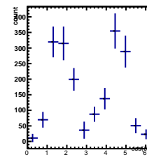
Raw Yields 4/5 < y < 5/5, -3.5/4.5 < \cos(\theta^*) < -2.5/4.5
