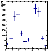
Raw Yields -5/5 < y < -4/5 , 1.5/4.5 < \cos(\theta^*) < 2.5/4.5
