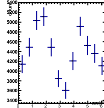
Raw Yields -3/5 < y < -2/5, -1.5/4.5 < \cos(\theta^*) < -0.5/4.5
