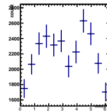
Raw Yields 3/5 < y < 4/5, -4.5/4.5 < \cos(\theta^*) < -3.5/4.5
