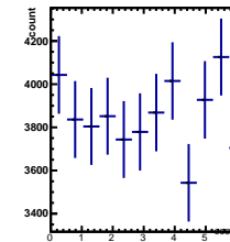
Raw Yields -1/5 < y < 0/5 , 3.5/4.5 < \cos(\theta^*) < 4.5/4.5
