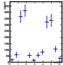
Raw Yields 4/5 < y < 5/5, 0.5/4.5 < \cos(\theta^*) < 1.5/4.5
