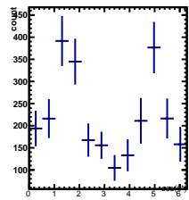
Raw Yields -5/5 < y < -4/5, -4.5/4.5 < \cos(\theta^*) < -3.5/4.5
