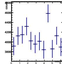
Raw Yields 0/5 < y < 1/5 , 2.5/4.5 < \cos(\theta^*) < 3.5/4.5
