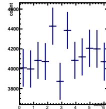
Raw Yields 1/5 < y < 2/5 , 2.5/4.5 < \cos(\theta^*) < 3.5/4.5
