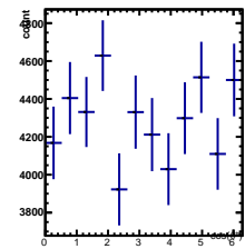
Raw Yields 0/5 < y < 1/5, -2.5/4.5 < \cos(\theta^*) < -1.5/4.5
