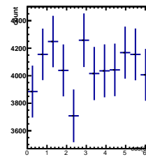
Raw Yields 1/5 < y < 2/5, -3.5/4.5 < \cos(\theta^*) < -2.5/4.5
