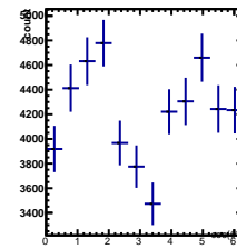
Raw Yields -3/5 < y < -2/5, -2.5/4.5 < \cos(\theta^*) < -1.5/4.5
