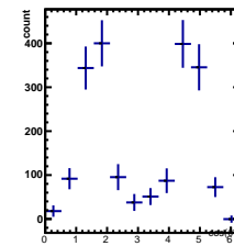
Raw Yields 4/5 < y < 5/5, -2.5/4.5 < \cos(\theta^*) < -1.5/4.5
