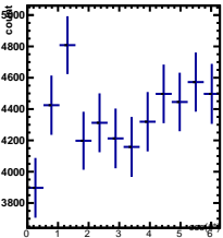
Raw Yields -1/5 < y < 0/5 , 1.5/4.5 < \cos(\theta^*) < 2.5/4.5
