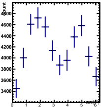
Raw Yields -3/5 < y < -2/5 , 1.5/4.5 < \cos(\theta^*) < 2.5/4.5
