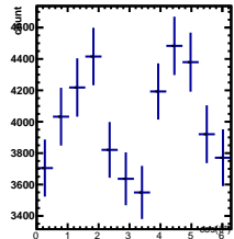
Raw Yields 2/5 < y < 3/5 , 1.5/4.5 < \cos(\theta^*) < 2.5/4.5
