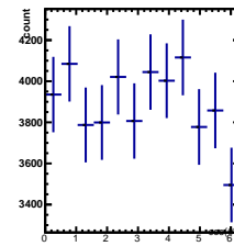
Raw Yields -1/5 < y < 0/5, -4.5/4.5 < \cos(\theta^*) < -3.5/4.5
