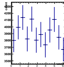
Raw Yields -3/5 < y < -2/5 , 3.5/4.5 < \cos(\theta^*) < 4.5/4.5
