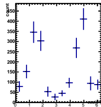
Raw Yields -5/5 < y < -4/5, -3.5/4.5 < \cos(\theta^*) < -2.5/4.5
