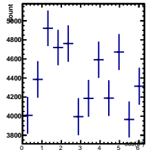
Raw Yields 0/5 < y < 1/5, 0.5/4.5 < \cos(\theta^*) < 1.5/4.5
