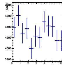
Raw Yields 1/5 < y < 2/5, -2.5/4.5 < \cos(\theta^*) < -1.5/4.5
