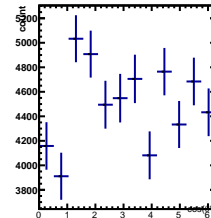
Raw Yields 1/5 < y < 2/5, -1.5/4.5 < \cos(\theta^*) < -0.5/4.5
