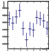
Raw Yields 1/5 < y < 2/5, 0.5/4.5 < \cos(\theta^*) < 1.5/4.5
