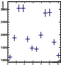
Raw Yields -4/5 < y < -3/5, 0.5/4.5 < \cos(\theta^*) < 1.5/4.5
