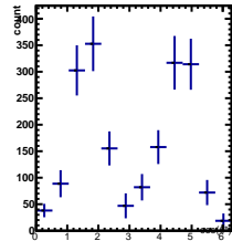
Raw Yields -5/5 < y < -4/5 , 2.5/4.5 < \cos(\theta^*) < 3.5/4.5
