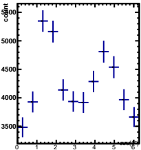
Raw Yields -3/5 < y < -2/5, 0.5/4.5 < \cos(\theta^*) < 1.5/4.5
