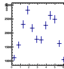
Raw Yields 3/5 < y < 4/5, -3.5/4.5 < \cos(\theta^*) < -2.5/4.5
