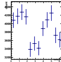
Raw Yields 2/5 < y < 3/5 , 2.5/4.5 < \cos(\theta^*) < 3.5/4.5
