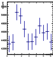
Raw Yields -1/5 < y < 0/5, -0.5/4.5 < \cos(\theta^*) < 0.5/4.5
