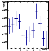
Raw Yields 1/5 < y < 2/5 , 1.5/4.5 < \cos(\theta^*) < 2.5/4.5
