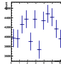
Raw Yields -1/5 < y < 0/5, -3.5/4.5 < \cos(\theta^*) < -2.5/4.5
