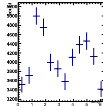
Raw Yields 2/5 < y < 3/5, -1.5/4.5 < \cos(\theta^*) < -0.5/4.5
