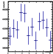
Raw Yields 0/5 < y < 1/5 , 1.5/4.5 < \cos(\theta^*) < 2.5/4.5
