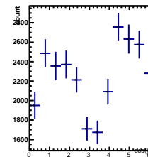
Raw Yields 3/5 < y < 4/5 , 3.5/4.5 < \cos(\theta^*) < 4.5/4.5
