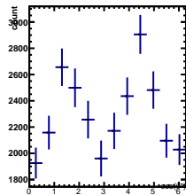
Raw Yields -4/5 < y < -3/5 , 3.5/4.5 < \cos(\theta^*) < 4.5/4.5
