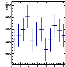
Raw Yields -2/5 < y < -1/5 , 2.5/4.5 < \cos(\theta^*) < 3.5/4.5
