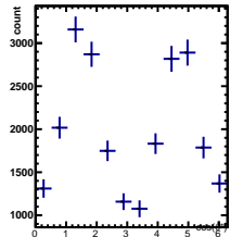
Raw Yields 3/5 < y < 4/5, 0.5/4.5 < \cos(\theta^*) < 1.5/4.5
