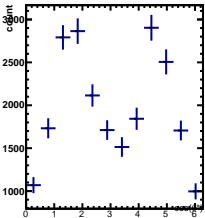
Raw Yields -4/5 < y < -3/5 , 1.5/4.5 < \cos(\theta^*) < 2.5/4.5
