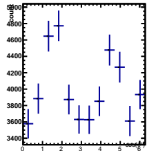
Raw Yields 2/5 < y < 3/5, 0.5/4.5 < \cos(\theta^*) < 1.5/4.5
