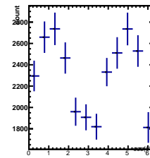
Raw Yields -4/5 < y < -3/5, -4.5/4.5 < \cos(\theta^*) < -3.5/4.5
