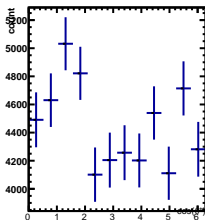
Raw Yields 0/5 < y < 1/5, -0.5/4.5 < \cos(\theta^*) < 0.5/4.5
