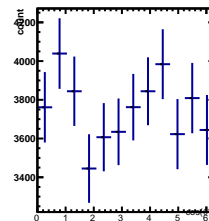
Raw Yields 2/5 < y < 3/5 , 3.5/4.5 < \cos(\theta^*) < 4.5/4.5
