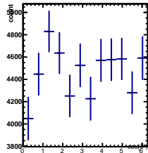
Raw Yields 0/5 < y < 1/5, -1.5/4.5 < \cos(\theta^*) < -0.5/4.5
