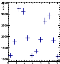
Raw Yields -4/5 < y < -3/5, -0.5/4.5 < \cos(\theta^*) < 0.5/4.5
