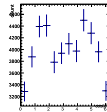
Raw Yields 2/5 < y < 3/5, -2.5/4.5 < \cos(\theta^*) < -1.5/4.5
