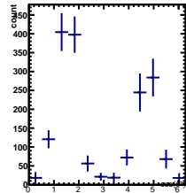
Raw Yields -5/5 < y < -4/5, -1.5/4.5 < \cos(\theta^*) < -0.5/4.5
