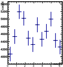
Raw Yields -2/5 < y < -1/5 , 1.5/4.5 < \cos(\theta^*) < 2.5/4.5
