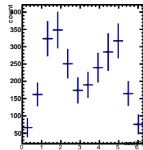
Raw Yields -5/5 < y < -4/5 , 3.5/4.5 < \cos(\theta^*) < 4.5/4.5
