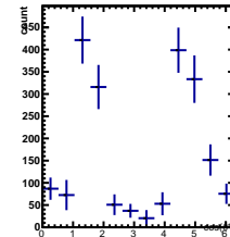
Raw Yields 4/5 < y < 5/5 , 2.5/4.5 < \cos(\theta^*) < 3.5/4.5
