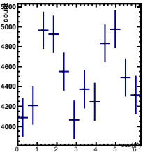
Raw Yields -1/5 < y < 0/5, 0.5/4.5 < \cos(\theta^*) < 1.5/4.5
