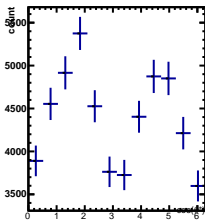
Raw Yields -3/5 < y < -2/5, -0.5/4.5 < \cos(\theta^*) < 0.5/4.5
