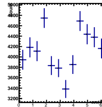
Raw Yields -3/5 < y < -2/5, -3.5/4.5 < \cos(\theta^*) < -2.5/4.5
