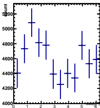
Raw Yields 1/5 < y < 2/5, -0.5/4.5 < \cos(\theta^*) < 0.5/4.5
