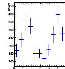
Raw Yields 4/5 < y < 5/5 , 3.5/4.5 < \cos(\theta^*) < 4.5/4.5
