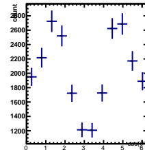
Raw Yields 3/5 < y < 4/5 , 2.5/4.5 < \cos(\theta^*) < 3.5/4.5
