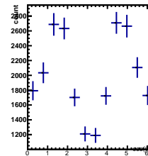
Raw Yields -4/5 < y < -3/5, -3.5/4.5 < \cos(\theta^*) < -2.5/4.5
