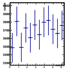
Raw Yields 0/5 < y < 1/5, -4.5/4.5 < \cos(\theta^*) < -3.5/4.5
