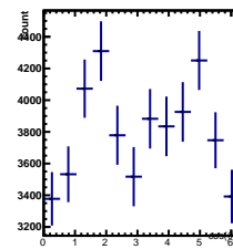
Raw Yields 2/5 < y < 3/5, -3.5/4.5 < \cos(\theta^*) < -2.5/4.5
