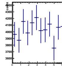
Raw Yields -2/5 < y < -1/5 , 3.5/4.5 < \cos(\theta^*) < 4.5/4.5
